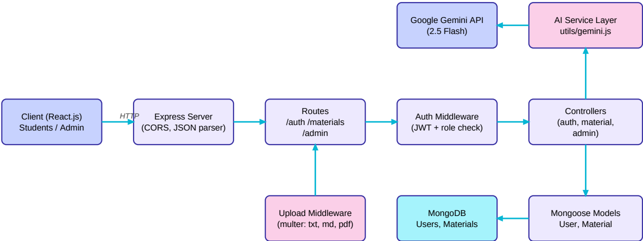
Technical architecture of AI StudyBuddy
